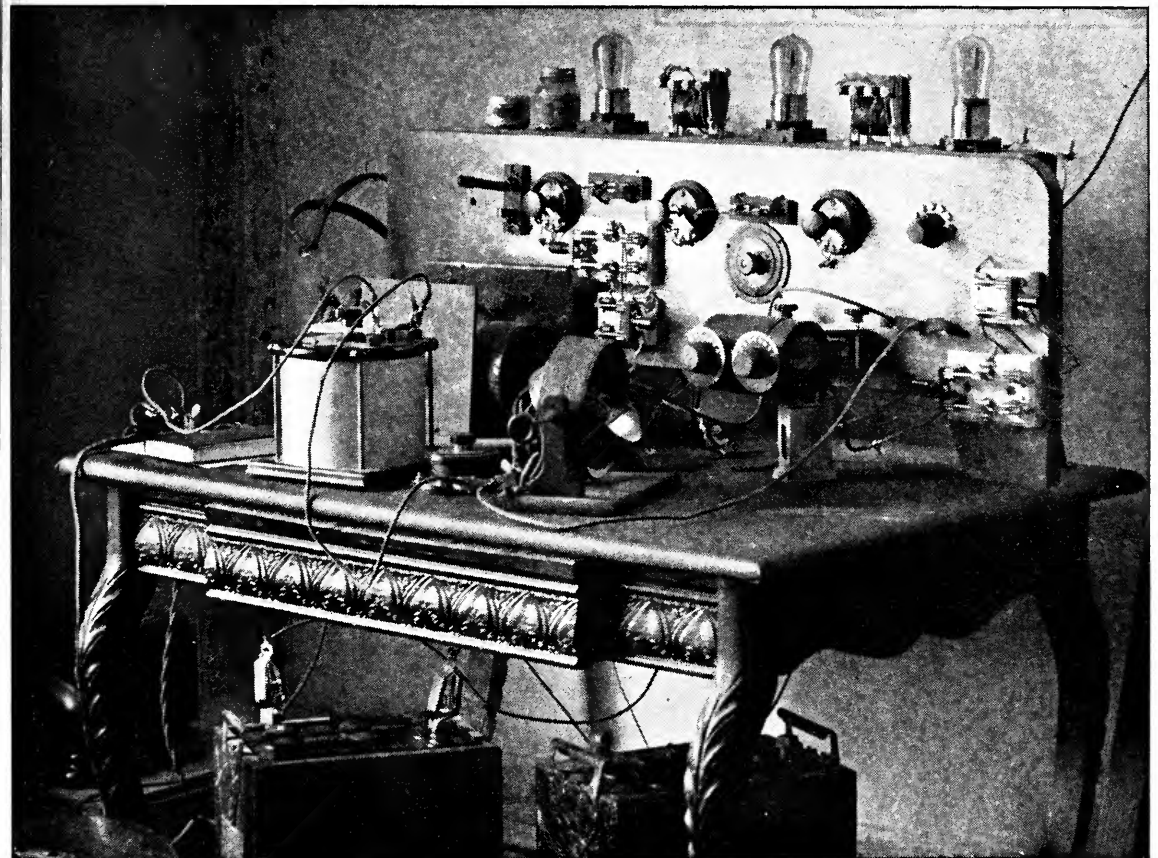
This Radio Regenerative Receiving Set, built by A. C. Philips, Hempstead, N. Y., has proved very effective. The antenna is composed of four strands of solid copper wire spaced two feet, eighty feet long, with a twenty-one foot lead-in. Height 51 feet. A home-made inductance wound on cardboard is used, with movable secondary, and taps on primary. A home-made variometer is used in the circuit as a tickler. The detector and two step amplification is made of standard parts. Double pole double throw switches connect to honey comb coils for long wave lengths. The following stations have been regularly and plainly heard. WJZ—WGI—WBZ—WGY—WWZ—KDKA—WDL—NOF—2XJ—IBKA—WYEB. The layout was arranged after a great deal of experimenting with different makes of standard parts, and left as shown owing to the fact that results were most satisfactory. Six sets of phones connected in series around the receiving room afford convenience and comfort to those who listen in.
