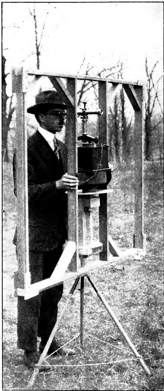
Radio direction finder frame on which telescope is mounted for use in sighting on the radio transmitting station. The scale of degrees is the circular disk just below the hand of the observer
